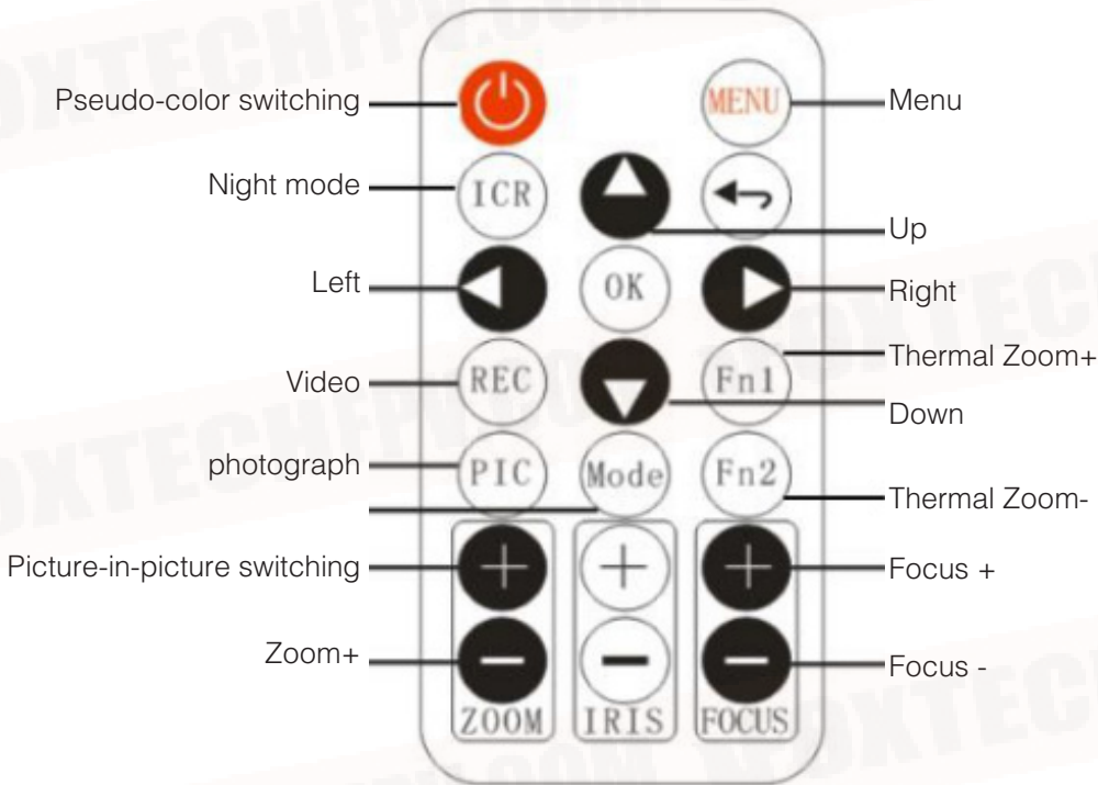
Infrared Remote Control Button Function
